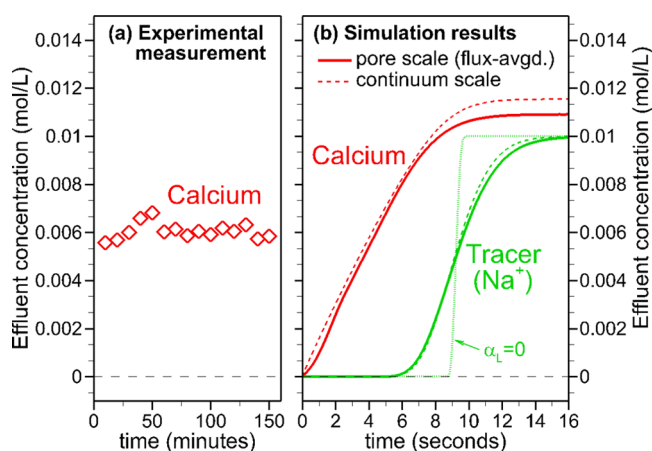
Figure 2. (a) Measured and (b) simulated effluent concentrations for calcium and a nonreactive tracer (sodium). Simulated concentrations consist of flux-averaged pore-scale simulation results and continuum-scale simulation results obtained using a longitudinal dispersivity ( \alpha_L ) equal to 0.012 cm. Tracer concentrations for a continuum-scale simulation with \alpha_L = 0 are also shown for reference. In contrast, the pore-scale simulation does not include any hydrodynamic dispersion, although molecular diffusion is considered.
