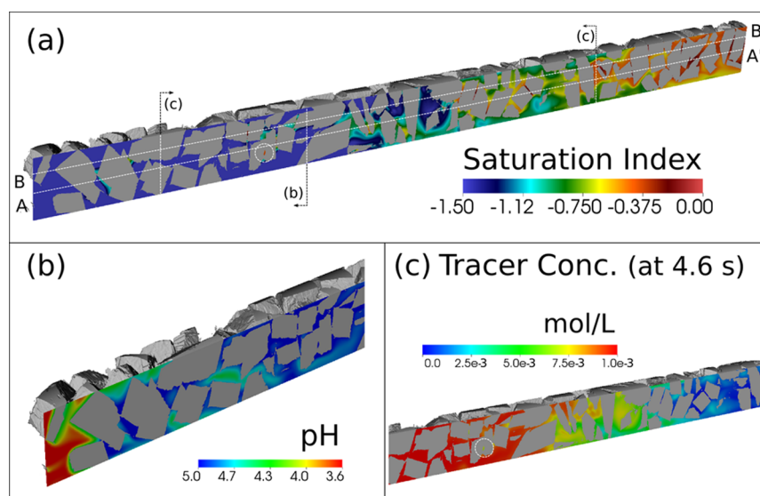
Figure 3. Selected geochemical results from the pore-scale simulation plotted on a plane that intersects the pore-scale domain, with the flow direction being from left to right: (a) Saturation index ( \log_{10} Q/K_S ) contours at 16 s showing the evolution from far-from-equilibrium conditions to near-equilibrium conditions, (b) pH contours at 16 s for the inlet portion the domain showing a significant diffusive boundary layer around the left-most grains, and (c) sodium concentrations in the capillary at 4.6 s, showing the mixing and spreading of the invasion front as well as isolated low-concentration pockets in small pore spaces left behind the front (an example is indicated by a dashed circle).
